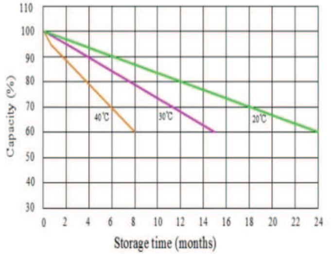
Self-discharge characteristic
