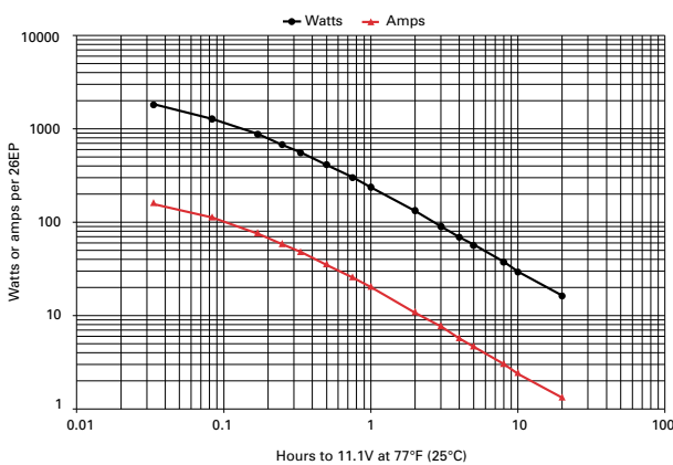
Figure B-12: 26EP discharge data to 11.1V at 77°F (25°C)
