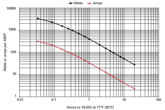
Figure B-14: 42EP discharge data to 10.02V at 77°F (25°C)
