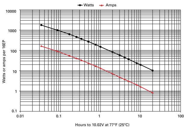
Figure B-6: 16EP discharge data to 10.02V at 77°F (25°C)
