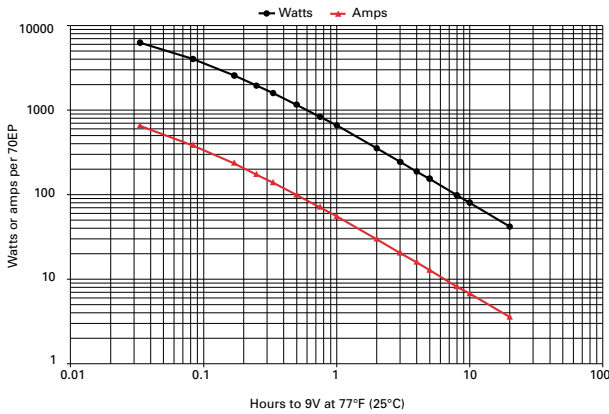
Figure B-17: 70EP discharge data to 9V at 77°F (25°C)
