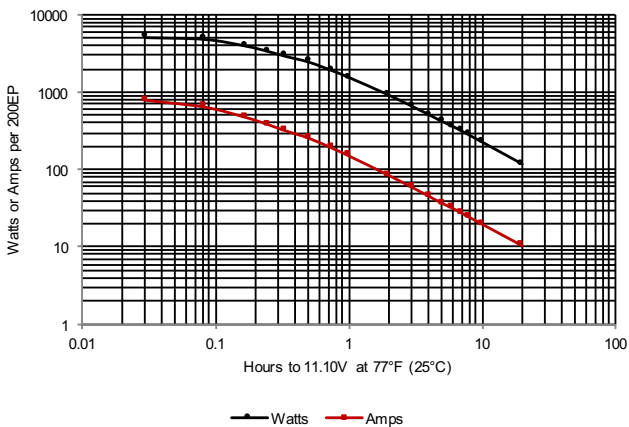
Figure B-24: 200EP Discharge data to 11.10V at 25°C (77°F)
