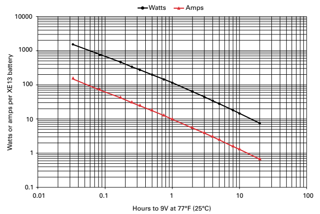
Figure A-1: XE13 discharge data to 9.0V at 77°F (25°C)
