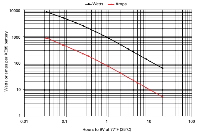
Figure A-25: XE95 discharge data to 9V at 77°F (25°C)
