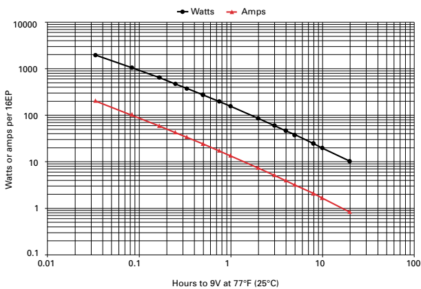
Figure B-5: 16EP discharge data to 9V at 77°F (25°C)
