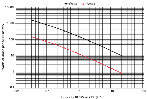
Figure A-6: XE16 discharge data to 10.02V at 77°F (25°C)
