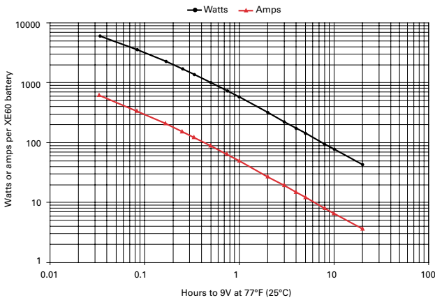
Figure A-17: XE60 discharge data to 9V at 77°F (25°C)
