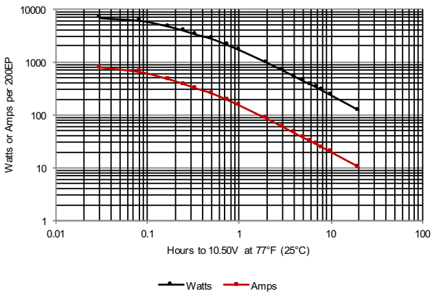
Figure B-23: 200EP Discharge data to 10.50V at 25°C (77°F)
