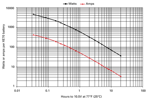
Figure A-23: XE70 discharge data to 10.5V at 77°F (25°C)
