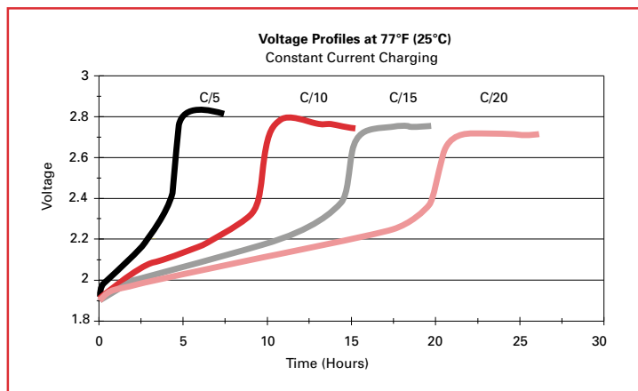
Figure 2.7.1: CC charging curves at 77°F (25°C)
