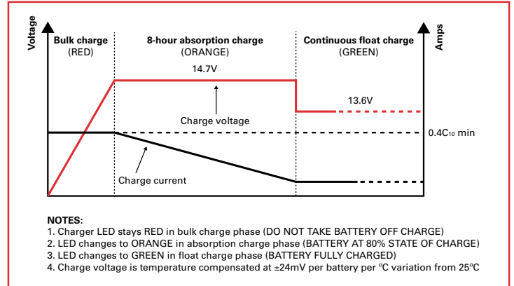
Figure 2.8.1: Three-step (IUU) charge profile
