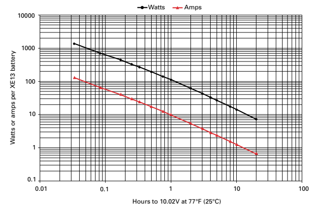
Figure A-2: XE13 discharge data to 10.02V at 77°F (25°C)
