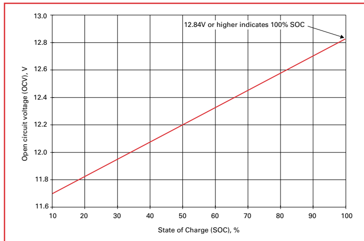
Figure 2.11.1: OCV and SOC
