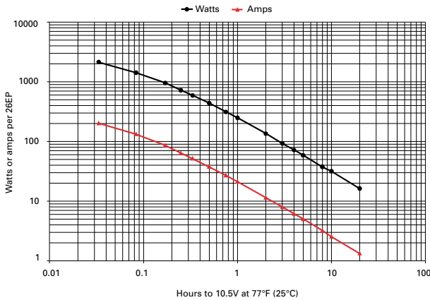
Figure B-11: 26EP discharge data to 10.5V at 77°F (25°C)
