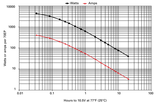
Figure B-19: 70EP discharge data to 10.5V at 77°F (25°C)
