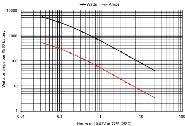
Figure A-18: XE60 discharge data to 10.02V at 77°F (25°C)
