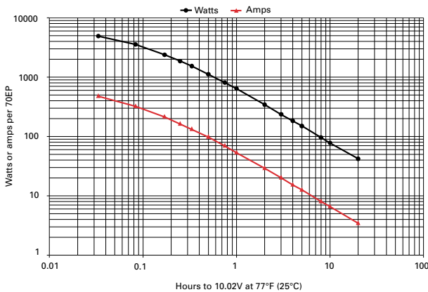
Figure B-18: 70EP discharge data to 10.02V at 77°F (25°C)
