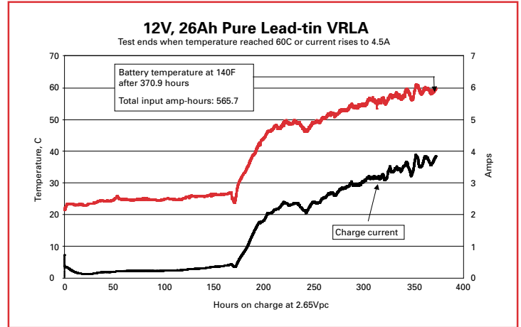
Figure 3.2.1: TR test at 15.9V (2.65Vpc) charge
