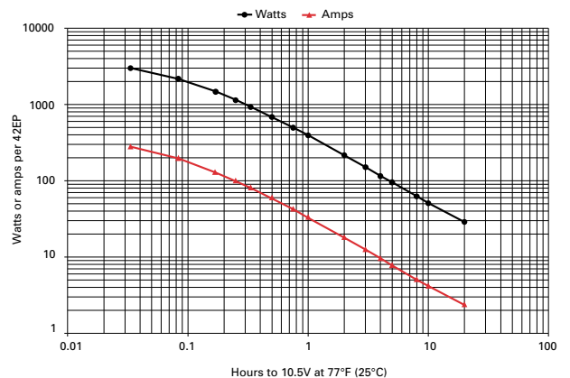
Figure B-15: 42EP discharge data to 10.5V at 77°F (25°C)
