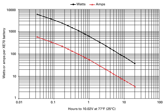
Figure A-22: XE70 discharge data to 10.02V at 77°F (25°C)
