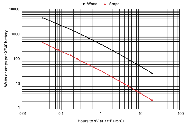
Figure A-13: XE40 discharge data to 9V at 77°F (25°C)
