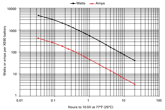
Figure A-19: XE60 discharge data to 10.5V at 77°F (25°C)
