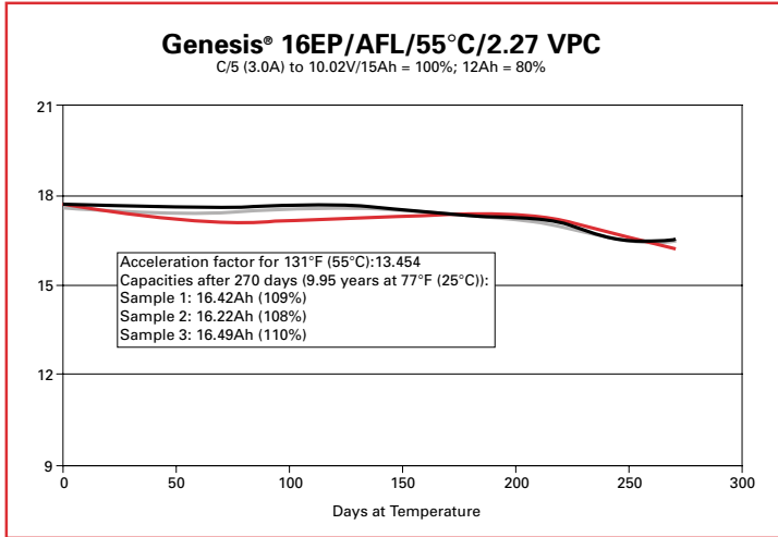
Figure 3.7.1: AFL test data for Genesis® 16EP batteries
