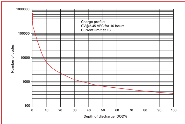
Figure 2.3.1: Cycle life and DOD
