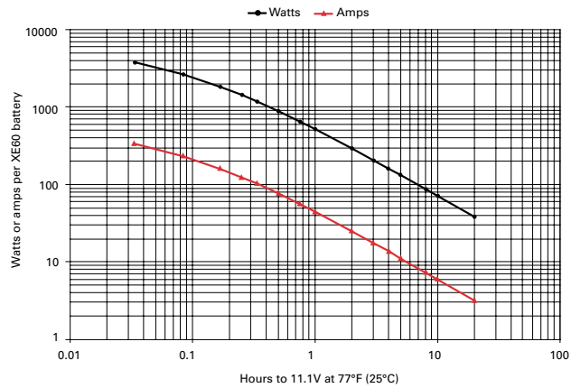
Figure A-20: XE60 discharge data to 11.1V at 77°F (25°C)
