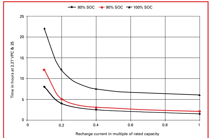
Figure 2.5.1: Recharge times under float charge
