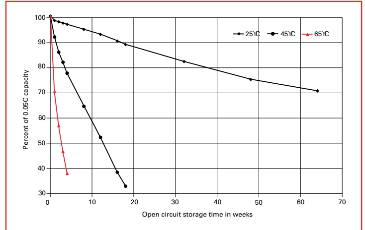
Figure 2.11.2: Storage capacity at temperatures
