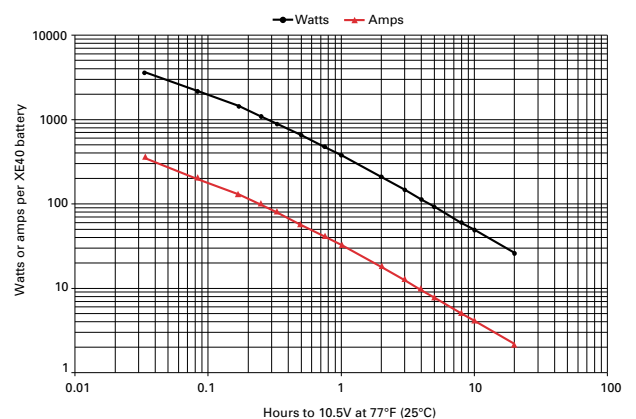
Figure A-15: XE40 discharge data to 10.5V at 77°F (25°C)
