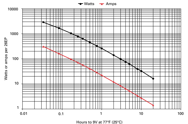
Figure B-9: 26EP discharge data to 9V at 77°F (25°C)
