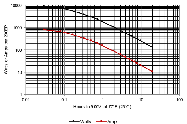
Figure B-21: 200EP Discharge data to 9.00V at 77°F (25°C)
