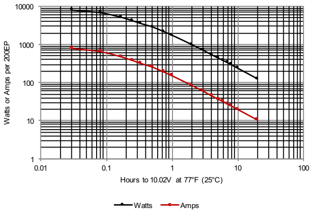
Figure B-22: 200EP Discharge data to 10.02V at 25°C (77°F)
