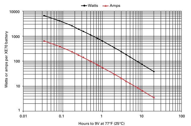
Figure A-21: XE70 discharge data to 9V at 77°F (25°C)
