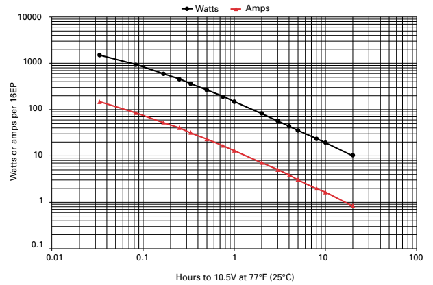
Figure B-7: 16EP discharge data to 10.5V at 77°F (25°C)
