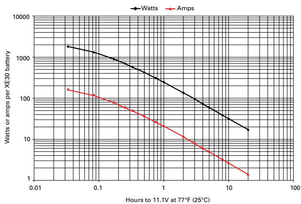
Figure A-12: XE30 discharge data to 11.1V at 77°F (25°C)
