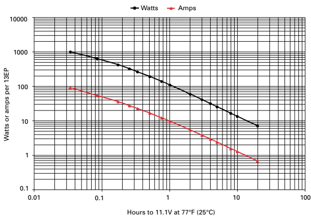
Figure B-4: 13EP discharge data to 11.1V at 77°F (25°C)
