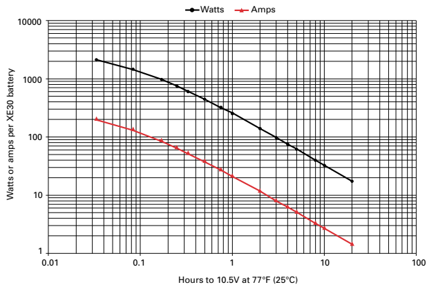
Figure A-11: XE30 discharge data to 10.5V at 77°F (25°C)
