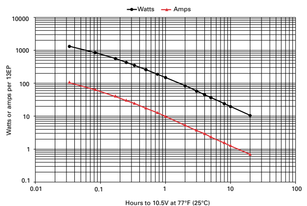
Figure B-3: 13EP discharge data to 10.5V at 77°F (25°C)
