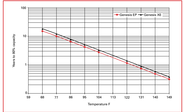
Figure 2.3.2: Battery temperature and float life
