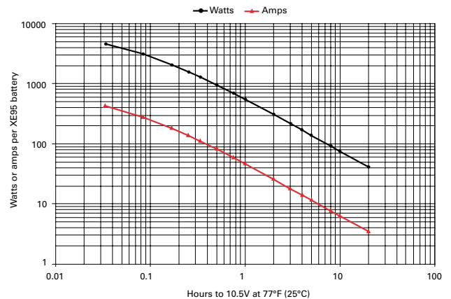
Figure A-27: XE95 discharge data to 10.5V at 77°F (25°C)
