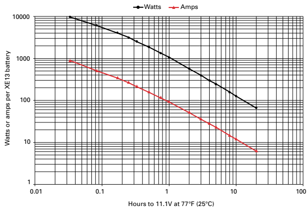
Figure A-4: XE13 discharge data to 11.1V at 77°F (25°C)
