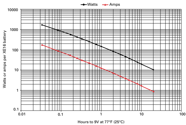
Figure A-5: XE16 discharge data to 9V at 77°F (25°C)
