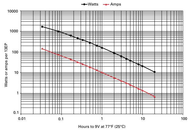
Figure B-1: 13EP discharge data to 9V at 77°F (25°C)
