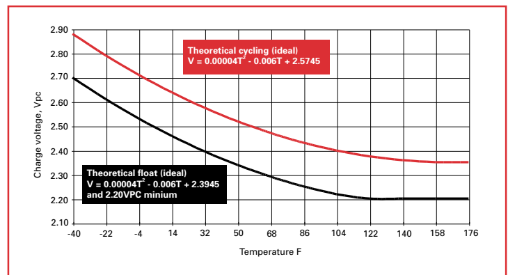
Figure 2.6.1: Temperature compensation graph
