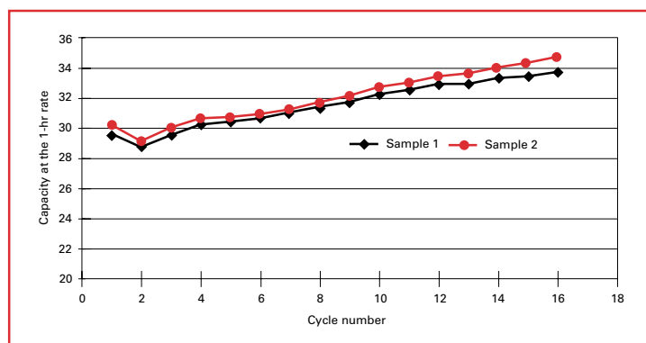
Figure 3.5.1: Recovery from discharged storage at 122°F (50°C)
