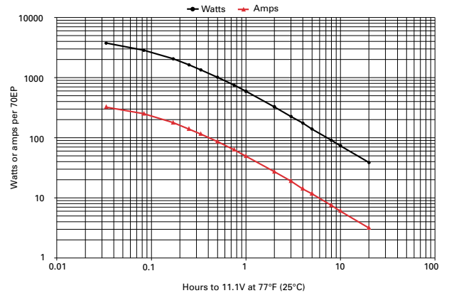
Figure B-20: 70EP discharge data to 11.1V at 77°F (25°C)
