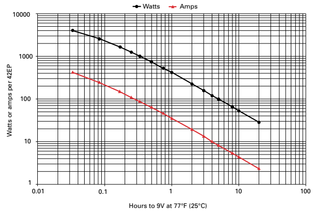
Figure B-13: 42EP discharge data to 9V at 77°F (25°C)
