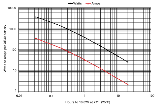
Figure A-14: XE40 discharge data to 10.02V at 77°F (25°C)
