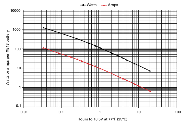
Figure A-3: XE13 discharge data to 10.5V at 77°F (25°C)
