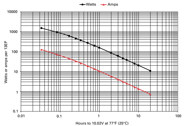
Figure B-2: 13EP discharge data to 10.02V at 77°F (25°C)
