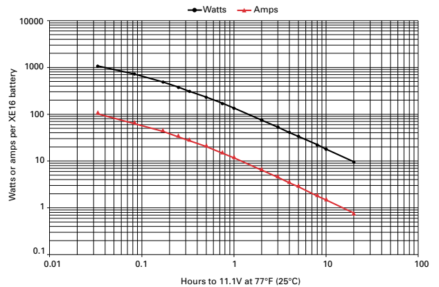
Figure A-8: XE16 discharge data to 11.1V at 77°F (25°C)
