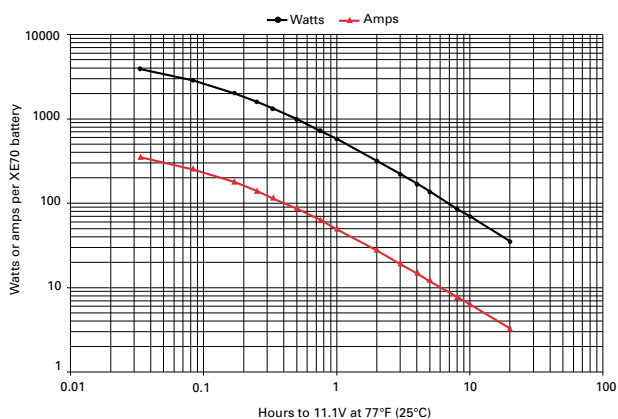
Figure A-24: XE70 discharge data to 11.1V at 77°F (25°C)
