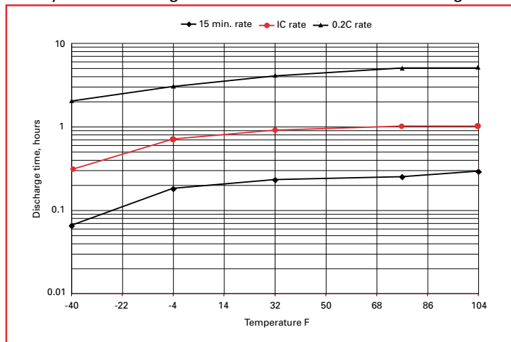
Figure 2.4.1: Capacity as a function of temperature
