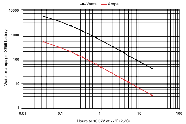
Figure A-26: XE95 discharge data to 10.02V at 77°F (25°C)
