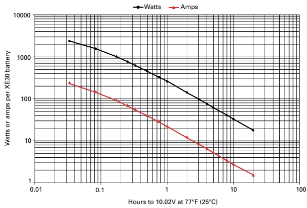
Figure A-10: XE30 discharge data to 10.02V at 77°F (25°C)
