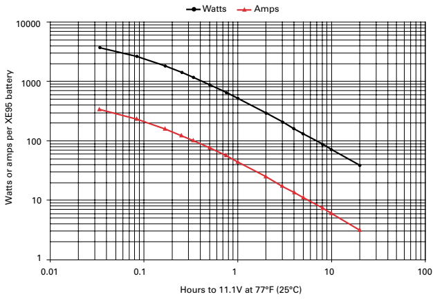
Figure A-28: XE95 discharge data to 11.1V at 77°F (25°C)
