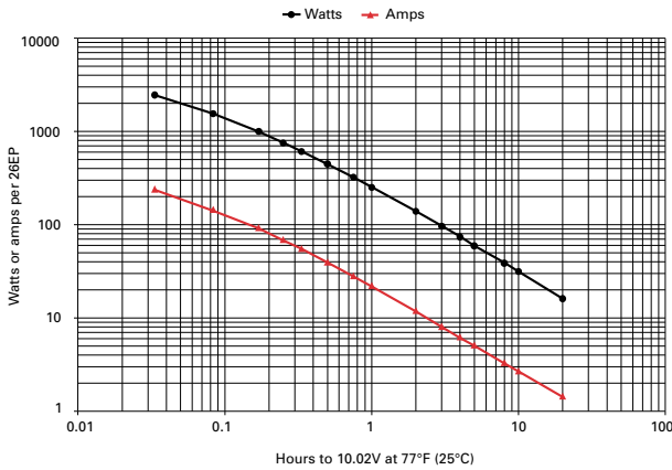
Figure B-10: 26EP discharge data to 10.02V at 77°F (25°C)
