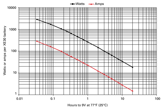
Figure A-9: XE30 discharge data to 9V at 77°F (25°C)
