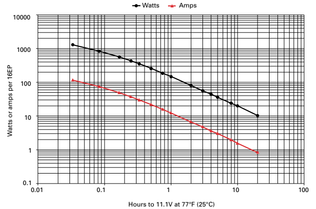
Figure B-8: 16EP discharge data to 11.1V at 77°F (25°C)
