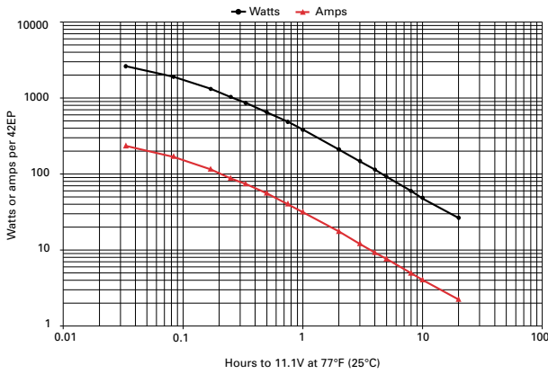
Figure B-16: 42EP discharge data to 11.1V at 77°F (25°C)
