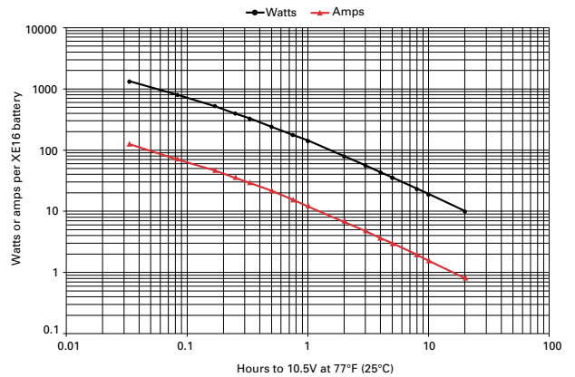
Figure A-7: XE16 discharge data to 10.5V at 77°F (25°C)
